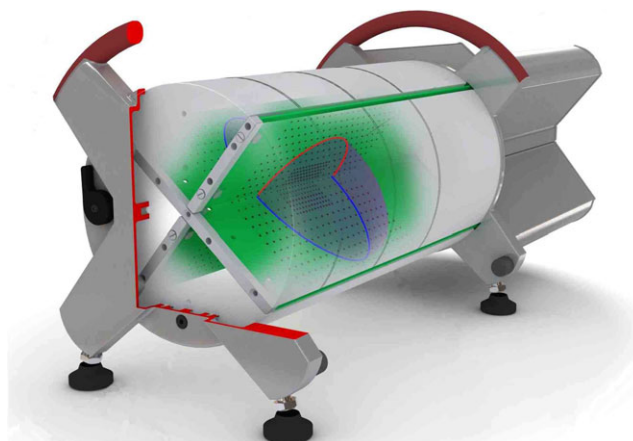
Fig. 1. Appearance of a 3D dose verification system (Delta4, ScandiDos). The silicon diodes are placed at 5 mm intervals in a central 6 cm × 6 cm area and at 10 mm intervals elsewhere in a 20 cm × 20 cm area on two orthogonal boards in the cylindrical phantom materials with a diameter of 22 cm. The standard detector geometry is depicted ("X"). If the attachment for sagittal-coronal option was used, the detector geometry could be rotated to the "+" orientation.
